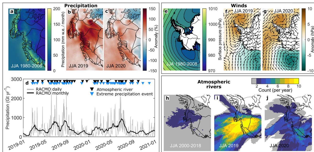
Fig. 5 | Precipitation anomalies during 2019 and 2020. a Winter (JJA) 1980–2008 climatology of monthly RACMO2.3p2 precipitation, and precipitation anomalies during b 2019 and c 2020. d Time-series of precipitation and timing of identified atmospheric rivers (black triangles) and extreme precipitation events (blue triangles) in 2019 and 2020. e JJA 1980–2008 climatology of daily ERA5 surface air
