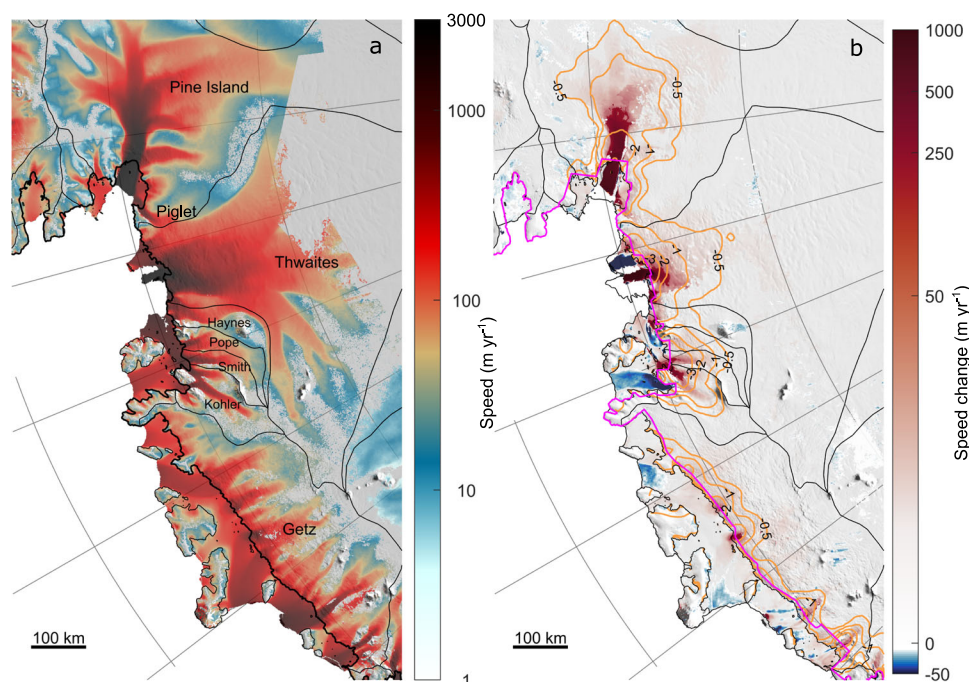
Fig. 1 | Ice speed and speed change in the Amundsen Sea Embayment.
