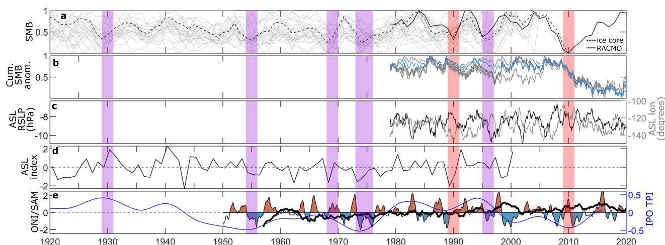
Fig. 6 | Potential historical snowfall droughts. a Normalised RACMO2.3p2 surface mass balance (SMB; solid black line) and normalised snow accumulation from 23 ice cores (grey lines; locations in Supplementary Fig. 9) and a West Antarctic Ice-Sheet composite 49 (dashed black line). b Normalised RACMO2.3p2 cumulative precipitation anomaly relative to the 1979–2008 mean, with individual basins (grey lines) and the total Amundsen Sea Embayment (blue line) shown. c Amundsen Sea Low (ASL) relative central pressure (black line) and centre
