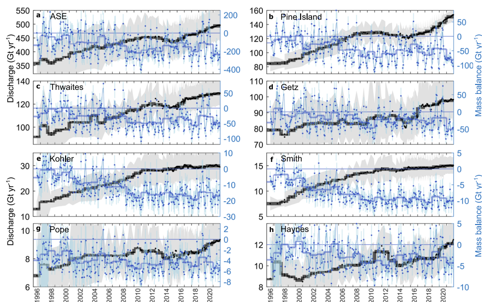
Fig. 2 | Grounding line discharge and mass balance timeseries. a–h Mass balance (blue) and grounding line discharge (black) from major Amundsen Sea Embayment basins. Individual observations are shown as filled markers with errors as vertical
