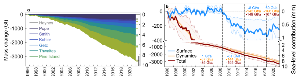
Fig. 3 | Cumulative mass change since 1996. a Cumulative mass change from major Amundsen Sea Embayment (ASE) basins, with sea-level equivalent shown on the right y-axis. Uncertainties are shown as floating bars after 2021—the grey bar indicates the total mass change uncertainty. b Cumulative mass changes
