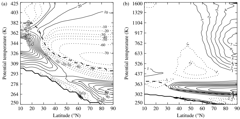
Figure 2. (a) The deviation from the reference state of the isentropic density, as a percentage of the reference isentropic density, (\sigma')/\sigma_{\text{ref}} \times 100\% , and (b) the deviation from the reference state of the scaled PV, Z_\theta (in PVU). The fields are plotted as a function of potential temperature (K) and latitude ( ^\circ\text{N} ) (note the different scales on the vertical axes). The contour interval is 10% for (a) and 1 PVU for (b), with the zero lines omitted and negative values indicated by thin dashed lines. The thick line near the lower boundary of the domain indicates the surface and the thick dashed line the tropopause (which is defined as the 2 PVU isopleth).
