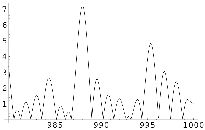
|\zeta(0.5+it)| , 980 < t < 1000
