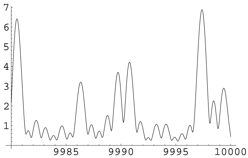
|\zeta(0.6+it)| , 9980 < t < 10000
