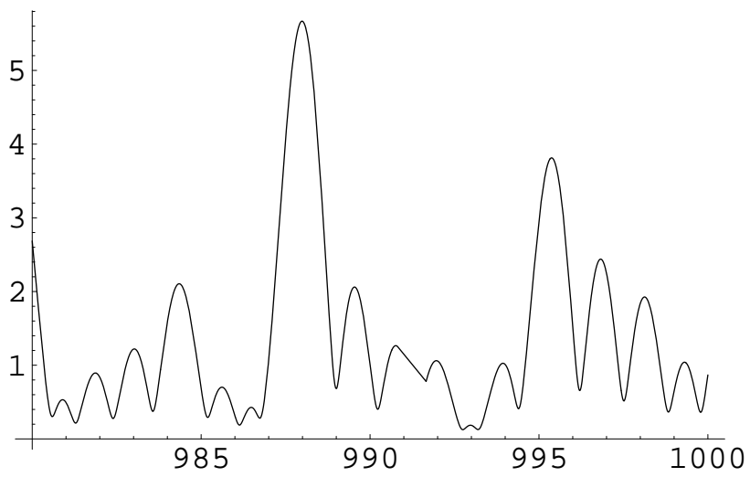
|\zeta(0.6+it)| , 980 < t < 1000
