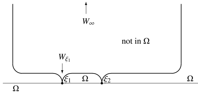
FIGURE 1. An \{\infty, \xi_1, \xi_2\} -excised neighbourhood.
