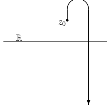
FIGURE 5 Both h_{\text{ri}} and h_{\text{le}} are solutions of (3.4) for E as in (3.7). We have for t \in \mathbb{R}
