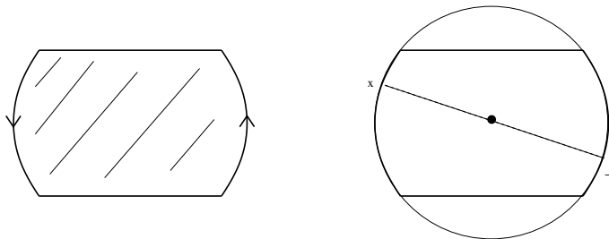
The Moebius band inside the projective plane
