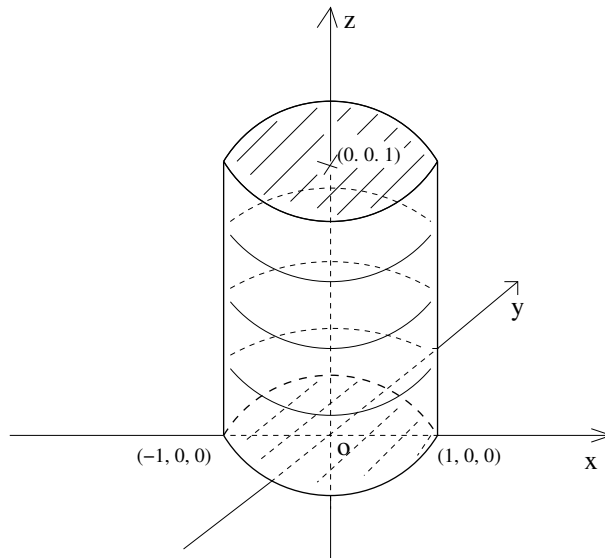
The cyclinder in \mathbb{R}^3
