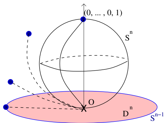
glue the boundary of D^n to a point to obtain S^n
