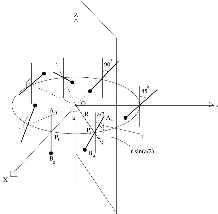
Explicit realization of the Moebius band in \mathbb{R}^3 : M_{R,r}
