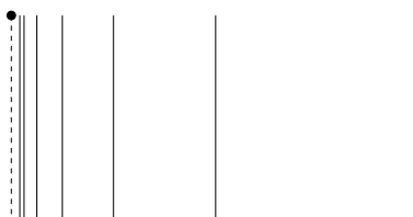
The flea and comb
