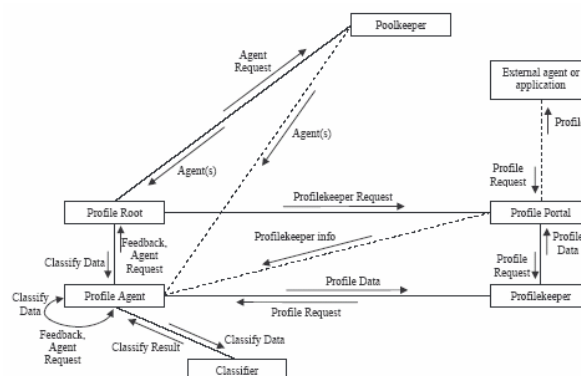
Fig. 3. The agent collaboration model
