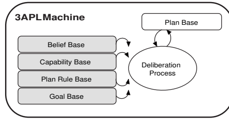
Fig. 2. 3APL Architecture
