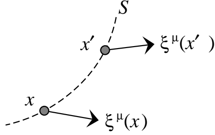
Figure 2: Two contravariant vectors close to each other on a curve S .
