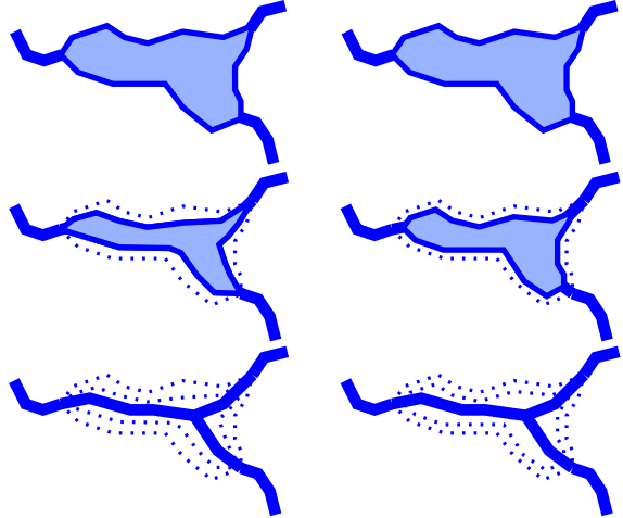
Figure 5: Collapsing an elongated lake into rivers.
