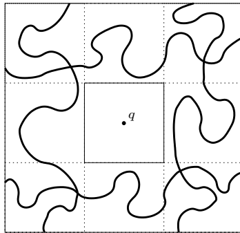
Figure 3: The event A_{q,r} .
