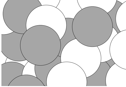
Figure 2: A close-up of a realization of the confetti process. Each cell is bounded by finitely many circle segments. There are points on the common boundary of three cells, but not of four.
