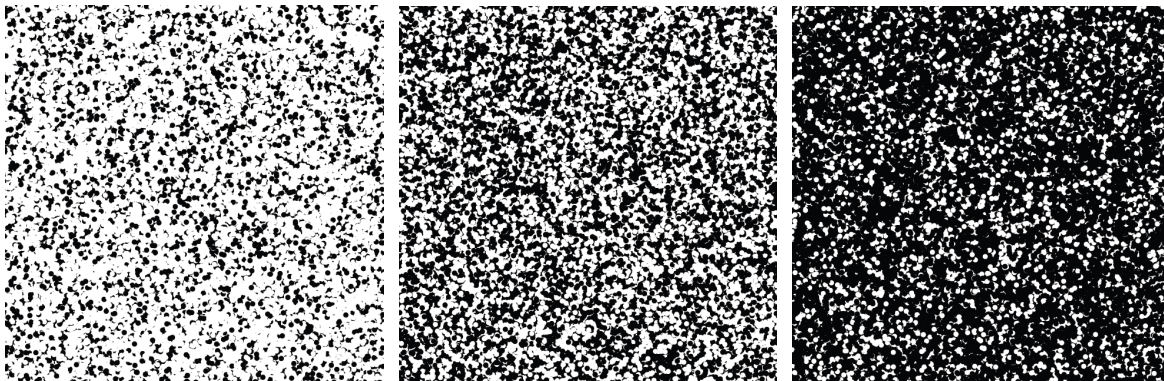
Figure 1: Simulations of confetti percolation with p = 1/4, 1/2, 3/4 . A square of dimensions 200 \times 200 is shown.
