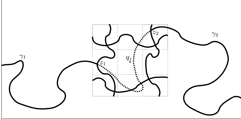
Figure 4: The curves \gamma_1 and \gamma_2 (not to scale).
