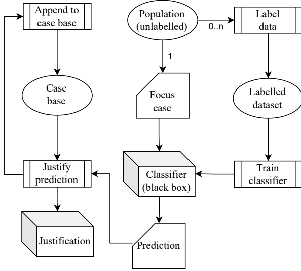
Figure 3: A schematic depiction of the context in which AF-CBA is applied without requiring access to the labelled dataset ( X ).
