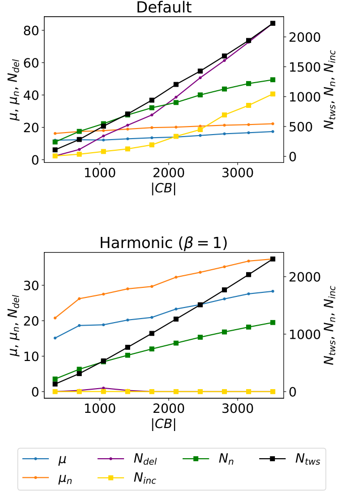
Figure 6: The various metrics as a function of the size of the CB in the data-agnostic approach for the churn dataset, averaged over three iterations for the default approach (top) and the harmonic ( \beta = 1 ) authoritativeness approach (bottom) to best precedent identification.
