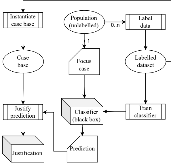
Figure 1: A schematic depiction of the context in which AF-CBA is applied.
