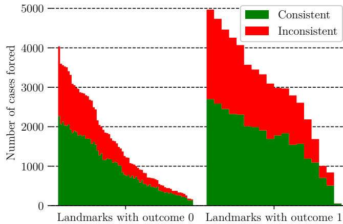
Figure 2. A visualization of the impact of the landmarks in the COMPAS data. Each vertical bar represents one landmark and shows the number of cases of which it forces the decision. The green area depicts the portion of those cases that have the same outcome as that landmark, and the red area the portion of cases which do not. Note that the leftmost bars are – by definition – the l_0 and l_1 cases of Definition 3.2, respectively.
