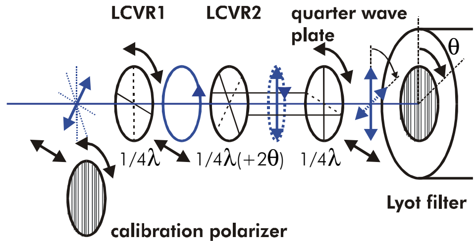
F.5.9. The design of the polarization modulation set-up.
