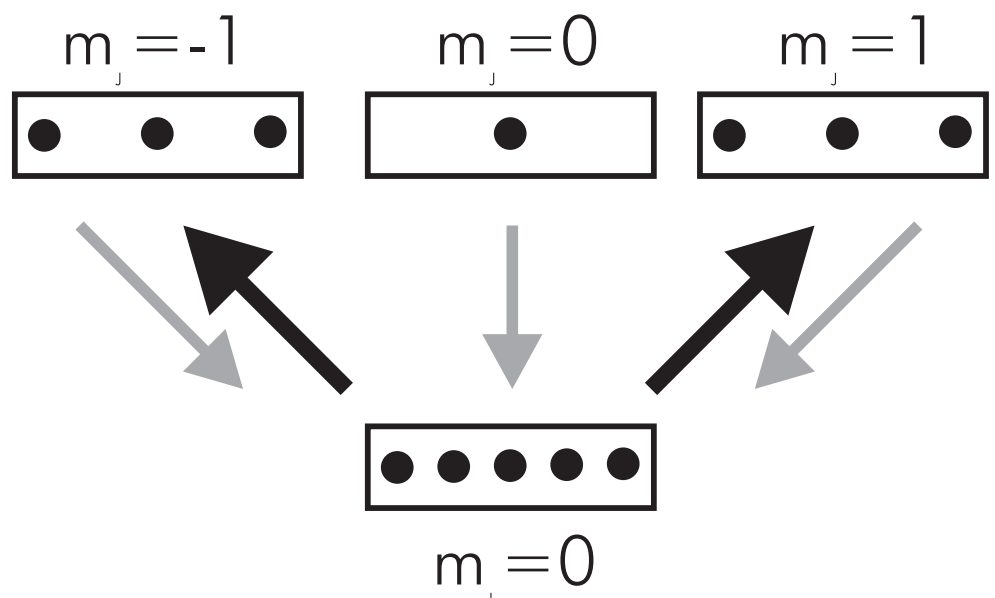
F.2.5. The creation of population imbalances in upper level quantum level substates by anisotropic illumination conform figure 2.4.b.
