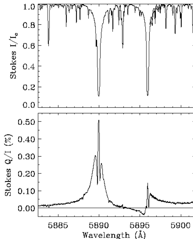
1 Na I D 2 and D 1
