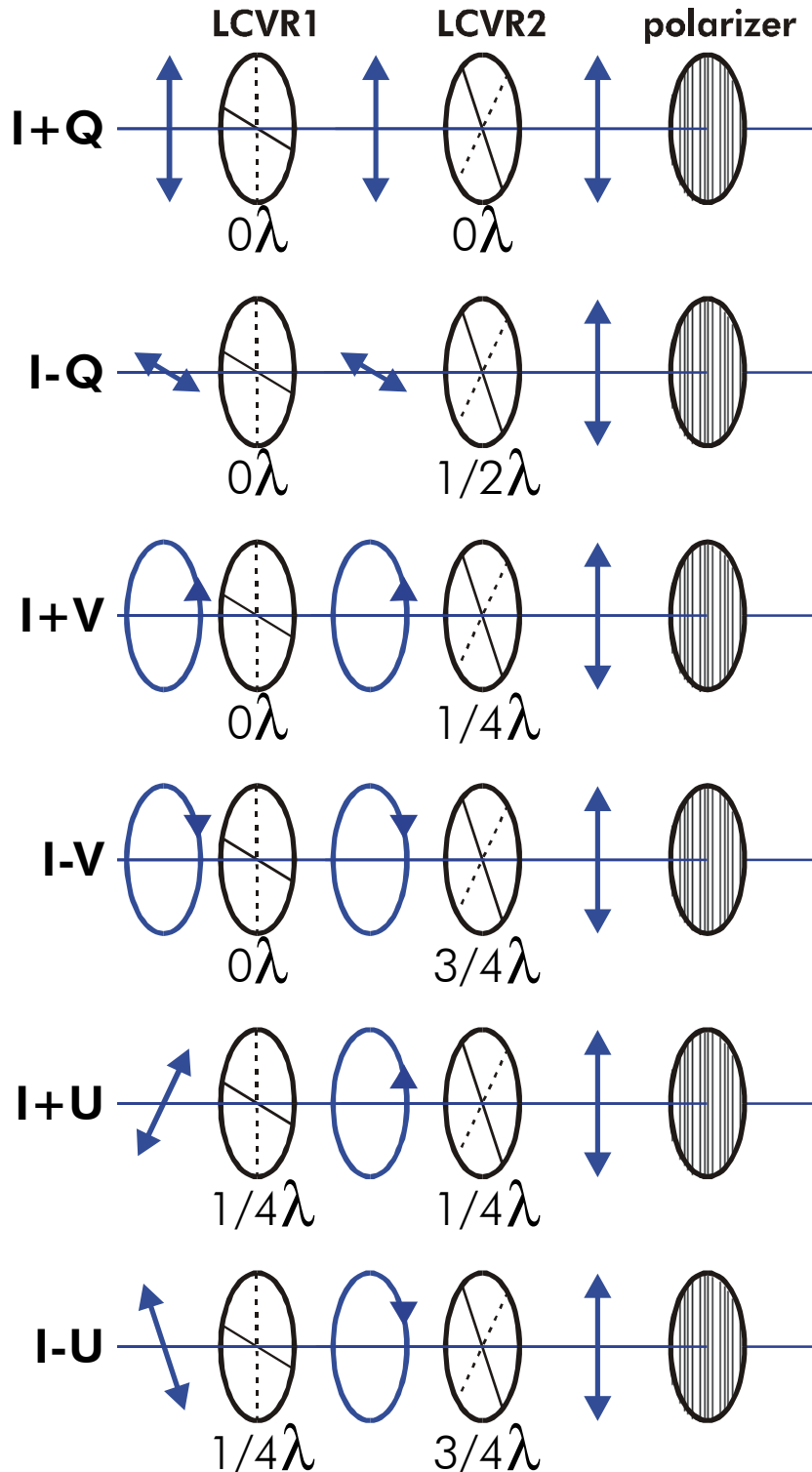
F.4.3. The measurement of the full Stokes vector with two LCVRs and a linear polarizer.
