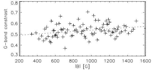
Fig. 9. G-band contrast vs field strength for the BP sample. The dashed line represents a linear fit to the data points.
