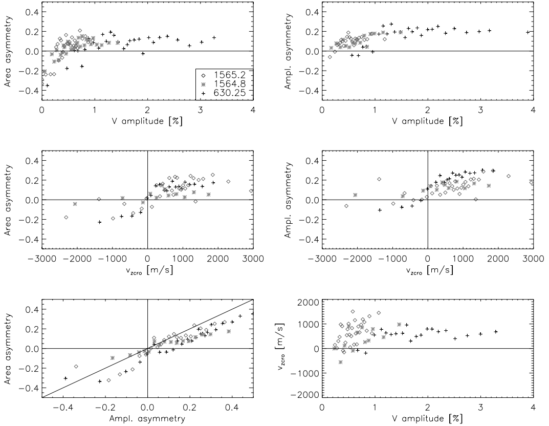
Fig. 15. Scatter plot of various Stokes V line parameters for the BP sample. Left to right, top to bottom: \delta A and \delta a vs. Stokes V amplitude, \delta A and \delta a vs. zero-crossing velocity, area asymmetry vs. amplitude asymmetry, and zero-crossing velocity vs. Stokes V amplitude.
