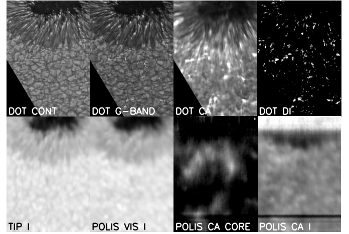
Fig. 1. Maps of the first scan across the limb-side part of NOAA 10425 after coarse alignment of DOT and VTT data. Top, left to right: blue continuum, G-band, and Ca II H line-core filtergrams from the DOT, and difference between the G-band and blue continuum images. Bottom, left to right: continuum intensity at 1.5 \mu\text{m} , continuum intensity at 630.4 \text{ nm} , intensity of the K_{2V} emission peak of the Ca II H line, and intensity in the Ca II H line wing; data from the VTT.
