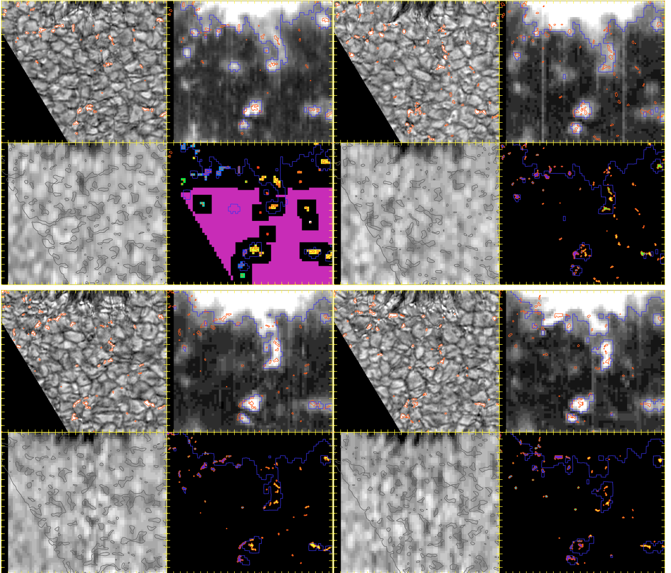
Fig. C.1. Coaligned maps from the VTT and the DOT for the first four repetitions of the scan. Clockwise, starting from top left of each 4 \times 4 subpanel: G-band intensity, total integrated polarization, DOT BP mask, and IR continuum intensity. Blue contours outline enhanced polarization signals and red contours the selected BP areas. In the DOT BP mask, the BPs are color-coded according to their number. The lower right map of the first 4 \times 4 subpanel is the VTT BP mask, not the DOT BP mask. In this map, the uniform pink area marks the spatial points used to extract the NBP sample. They are located outside the canopy, and at least 3 pixels ( 1''.05 ) away from any BP.
