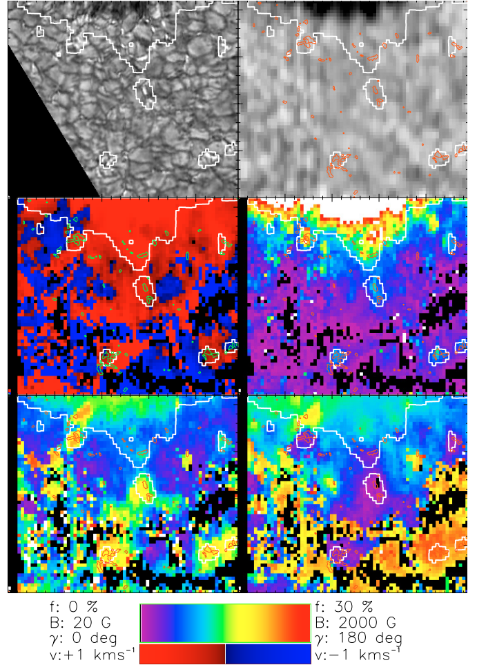
Fig. 5. Atmospheric parameters deduced from the inversion of the seventh map. Top: G-band intensity and IR continuum intensity. Middle: LOS velocity of the magnetic component and magnetic filling factor. Bottom: field strength and field inclination to the LOS. White contours outline areas of enhanced polarization signal and red contours (green in the velocity map) the identified BPs. Tickmarks are arcsec. Black areas represent pixels without polarization signal that have not been inverted in terms of a two-component model.
