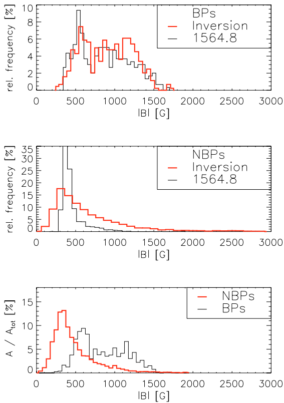
Fig. 8. Top: distribution of BP field strengths as inferred from the inversion (thick line) and the splitting of the Fe I 1564.8 nm line (thin line). Middle: same for the NBP sample. Bottom: fraction of the total area occupied by fields of given strength.
