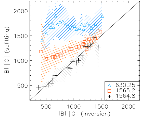
Fig. 7. Magnetic field strength of BPs from the Zeeman splitting of Fe I 1564.8 nm (+), 1565.2 nm ( \square ), and 630.25 nm ( \triangle ), vs. the values inferred from the inversion. The shaded areas give the scatter inside the bins. The straight line indicates a one-to-one correspondence.
