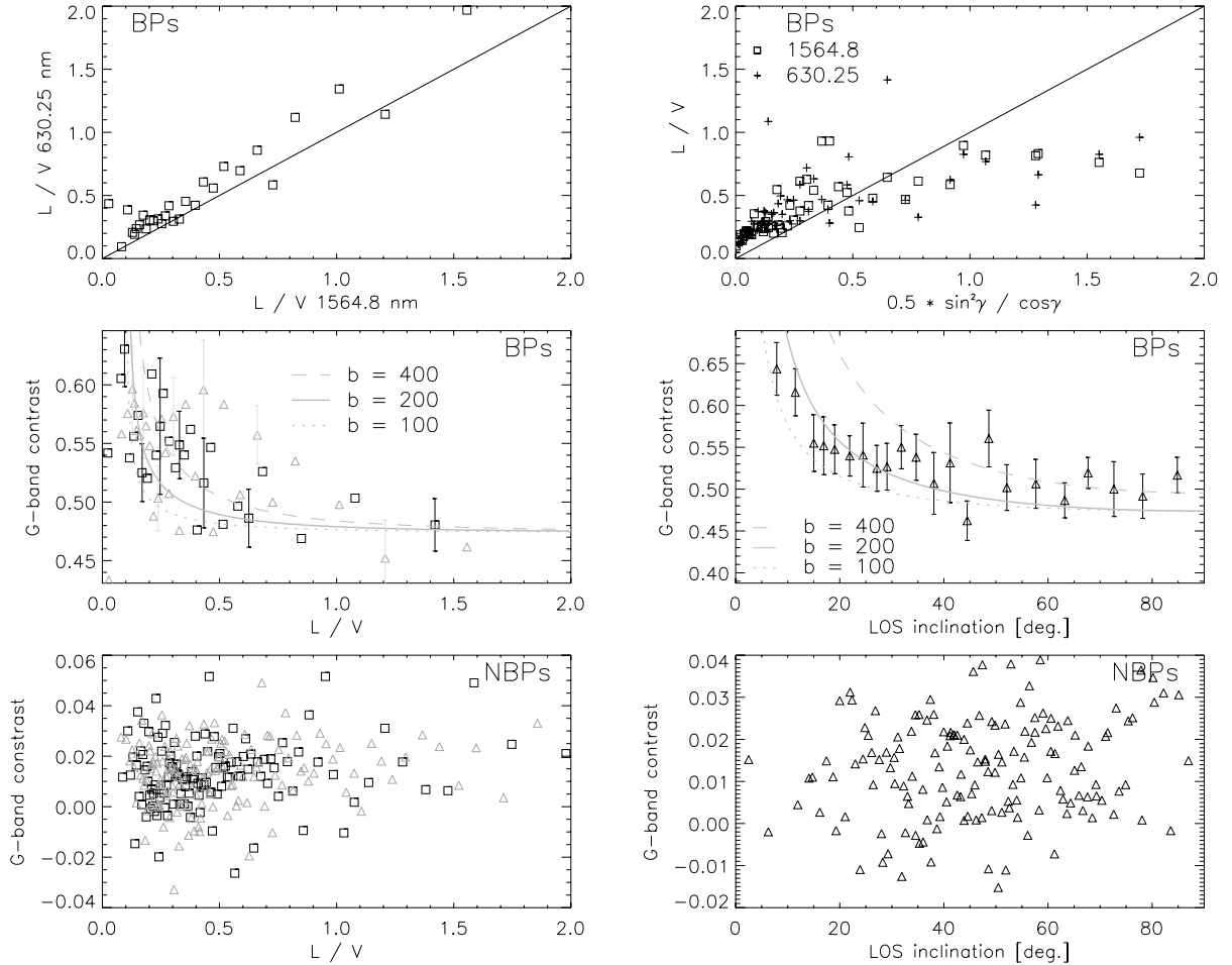
Fig. 11. Top panels: L/V of Fe I 630.25 nm vs. the L/V of Fe I 1564.8 nm (left), and L/V of 1564.8 nm ( \square ) and 630.25 nm ( + ) vs. the values obtained from Eq. (9) by inserting the inclinations deduced from the inversion (right). Middle left panel: dependence of the BP contrast on the L/V ratio of 1564.8 nm ( \triangle ) and on the L/V ratio averaged over the two visible lines ( \square ). Middle right panel: dependence of the BP contrast on the field inclination deduced from the inversion. Overplotted are curves calculated from Eq. (11) for three values of the parameter b . Error bars indicate the uncertainty of the mean values. Bottom panels: BP contrast vs. L/V and vs. inclination, for NBPs.
