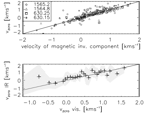
Fig. 13. Top: Stokes V zero-crossing velocity, v_{\text{zero}} , vs. the magnetic velocity from the inversion, for BPs. Bottom: BP zero-crossing velocities deduced from IR lines vs. those from visible lines. The zero-crossing velocity is averaged over the two visible (or infrared) lines when both show regular Stokes V profiles. The shaded area indicates the scatter in the bins.
