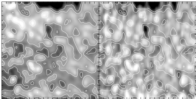
Fig. 2. Continuum intensity maps from POLIS (630 nm; left ) and TIP (1565 nm; right ). Only the lower part of the FOV is shown. Contours outline the brightest granules and darkest intergranular lanes observed in the POLIS map. Tick marks are separated by 1'' .
