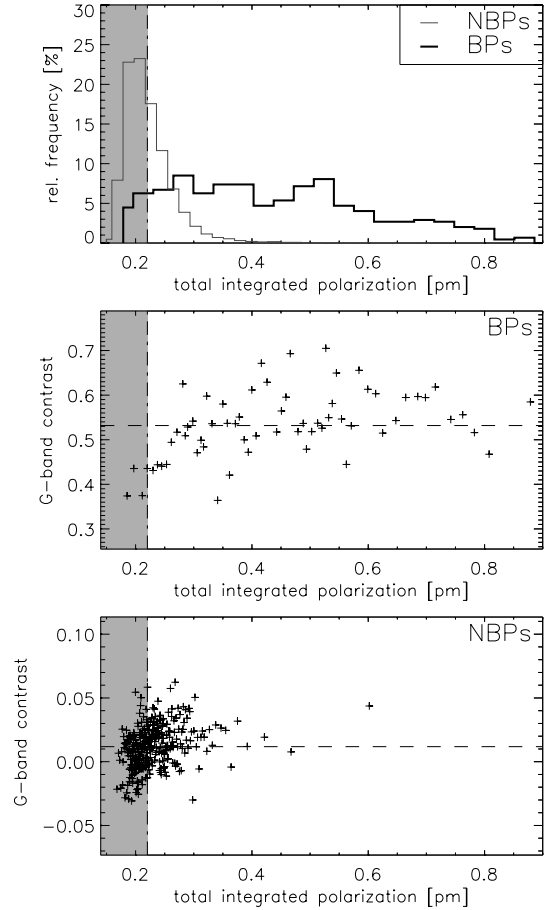
Fig. 6. Top: relative frequency of total integrated polarization values for BPs ( thick black ) and NBPs ( thin grey ). Middle and bottom: G-band contrast vs total integrated polarization for BPs and NBPs. The dashed horizontal lines indicate the mean contrast of 0.52 for BPs and 0.01 for NBPs. The shaded areas denote the range of \mathcal{T} values within the noise level.
