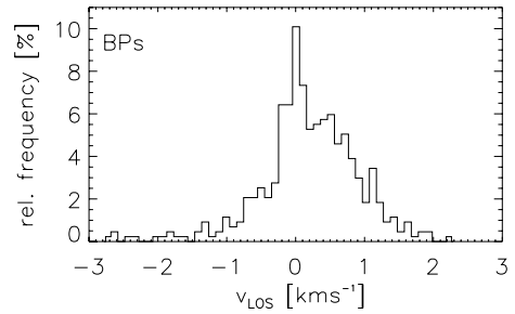
Fig. 14. Histogram of the LOS velocity of the magnetic component of the inversion, for BPs.
