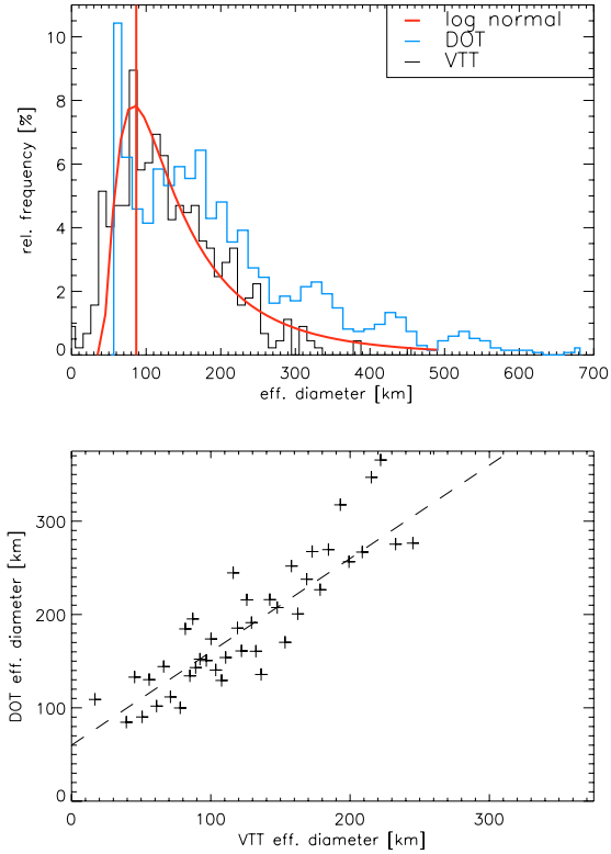
Fig. 19. Top: histogram of BP effective diameters from the VTT (thin black line) and the DOT (thick line). Overplotted is a log-normal distribution. Bottom: effective diameters from the DOT vs. those from the VTT. The dashed line has unity slope and 60 km offset.
