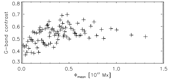
Fig. 16. G-band contrast vs. average single-pixel magnetic flux of BPs. The curve has a similar shape to the contrast vs. total integrated polarization (cf. Fig. 6).
