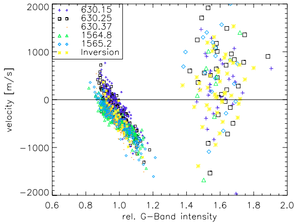
Fig. 12. Relation between the LOS velocity and the normalized G-band intensity. Positive velocities indicate redshifts. Small symbols: Stokes I line-core velocity and LOS velocity of the field-free component of the inversion for the NBP sample. Large symbols: Stokes V zero-crossing velocity and LOS velocity of the magnetic component of the inversion for BPs.
