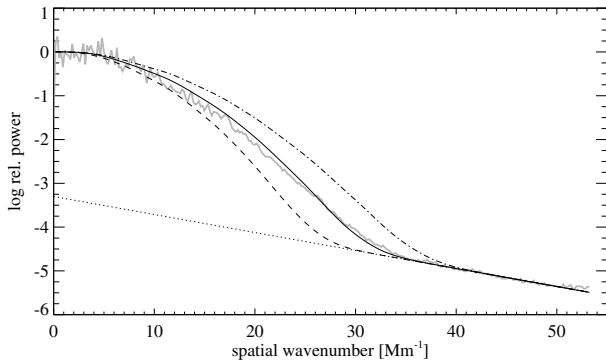
Fig. 3. Spatial power spectra for the penumbral intensity variations. The observed one is given by the thick grey line, the solid line represents the model with a typical width of 250 km, the dashed line stands for 290 and the dash-dotted line for 220 km. The straight dashed line shows the noise level.
