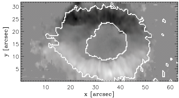
Fig. 5. Map of Doppler velocities. Velocities vary in a spectral sequence from -3.5 km/s (towards observer, black) to +3.5 km/s (white), grey indicates no or small Doppler shift.
