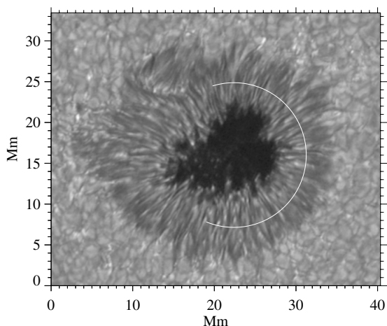
Fig. 1. A G-band image of the spot, obtained at the DOT. This image has been corrected for projection effects. The white line indicates the arc where the data for the spatial power spectra have been extracted.
