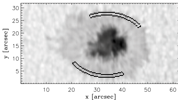
Fig. 2. Image of the spot composed from the Stokes-I spectra obtained during the scan. The surrounded areas in the outer penumbra are selected for the correlation analysis in section 5. The ordinate is parallel to the direction to disk centre.
