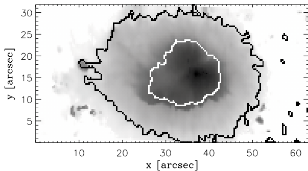
Fig. 4. Map of the magnetic field strength B . If the net polarization drops below a certain limit, the value of B is set to zero (white). The contours give the outer edge of the penumbra in the continuum and the umbra-penumbra boundary ( 0.83\% I_c ). Black corresponds to 3000 G.
