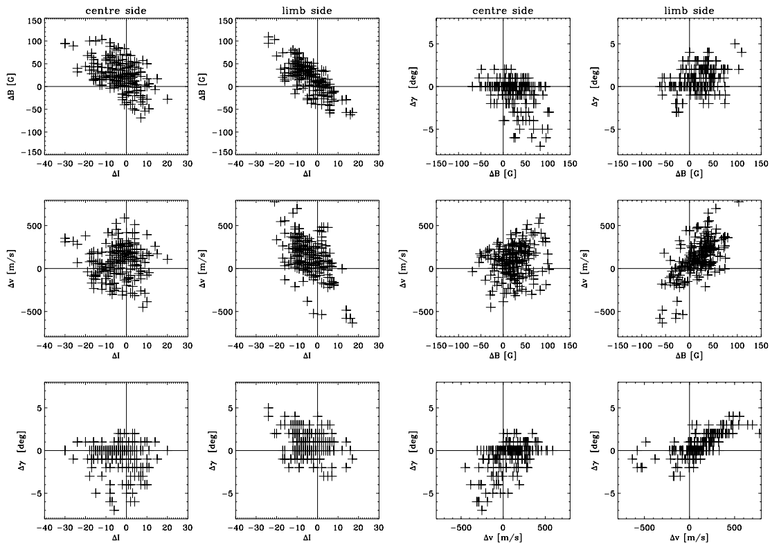
Fig. 6. Scatter plots for the relations of the variations of intensity and magnetic field (upper left panels), intensity and velocity (middle left panels), intensity and magnetic inclination (lower left panels), magnetic field strength and inclinations (upper right panels), magnetic field strength and velocities (middle right panels) and velocities and magnetic inclination (lower right panels). The first and third columns stand for the centre-side penumbra, the second and fourth for the limb-side penumbra.
