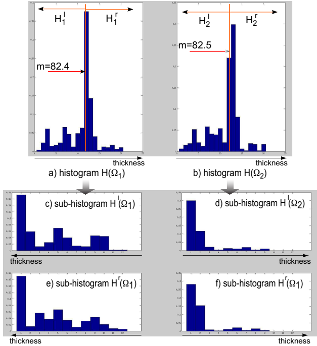
Figure 4: Median value separation histogram-distance d_{MV} .
