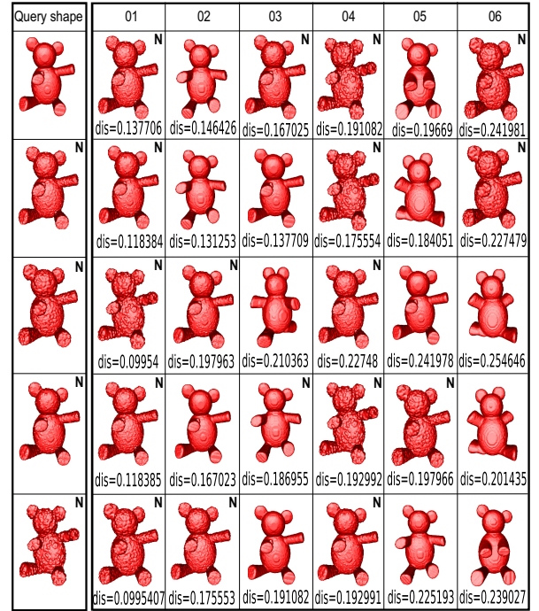
Figure 8: Retrieval robustness in presence of noise. Shapes marked ‘N’ contain artificially-added noise.
