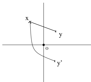
\mathbb{R}^2 - \{0\} is path connected
