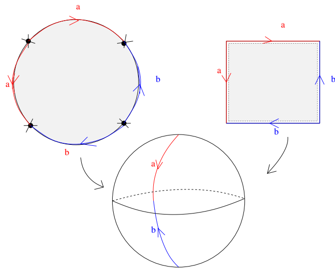
The sphere obtained from a disk or a square glueing as indicated in the pictu
