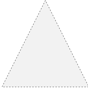
X= an open triangle
