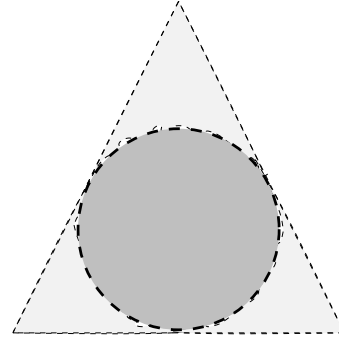
A= an open disk inside X
