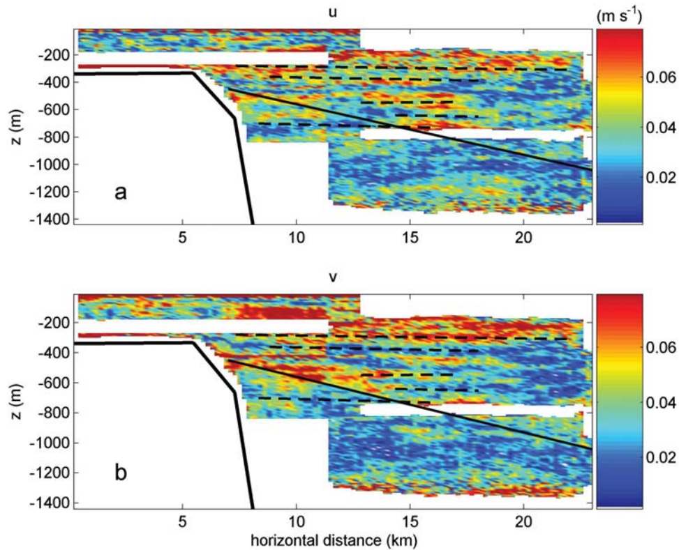
Figure 9. As Figure 6, but for GMS. Note the different color-scale compared to BB.
