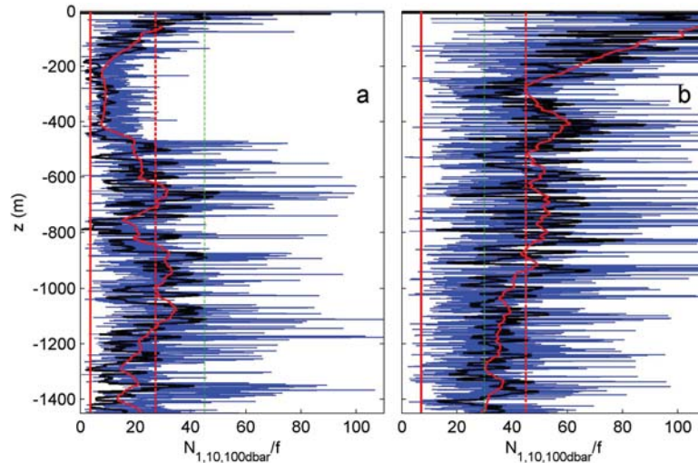
Figure 7. (a) Buoyancy frequency scaled with local inertial frequency and computed from CTD data obtained at horizontal distance 18 km in BB (end of second track, at a depth of 1720 m) over vertical scales \Delta z = 1 (blue), \Delta z = 10 (black) and \Delta z = 100 (red) m. The vertical red lines indicate lower limit N = 4f_h (red solid line), 27f (mean N for depth-range 500–1200 m; red-dashed) and 45f (upper-limit, mean value GMS; green-dashed lines). (b) As (a), but for GMS-data during yoyo-station at horizontal distance 12 km in towed transect, two weeks later. Here vertical lines at 27f (minimum-mean, mean value BB; green dashed) and 45f (mean for depth-range 500–1200 m; red-dashed). All N -values are excluding instabilities.
