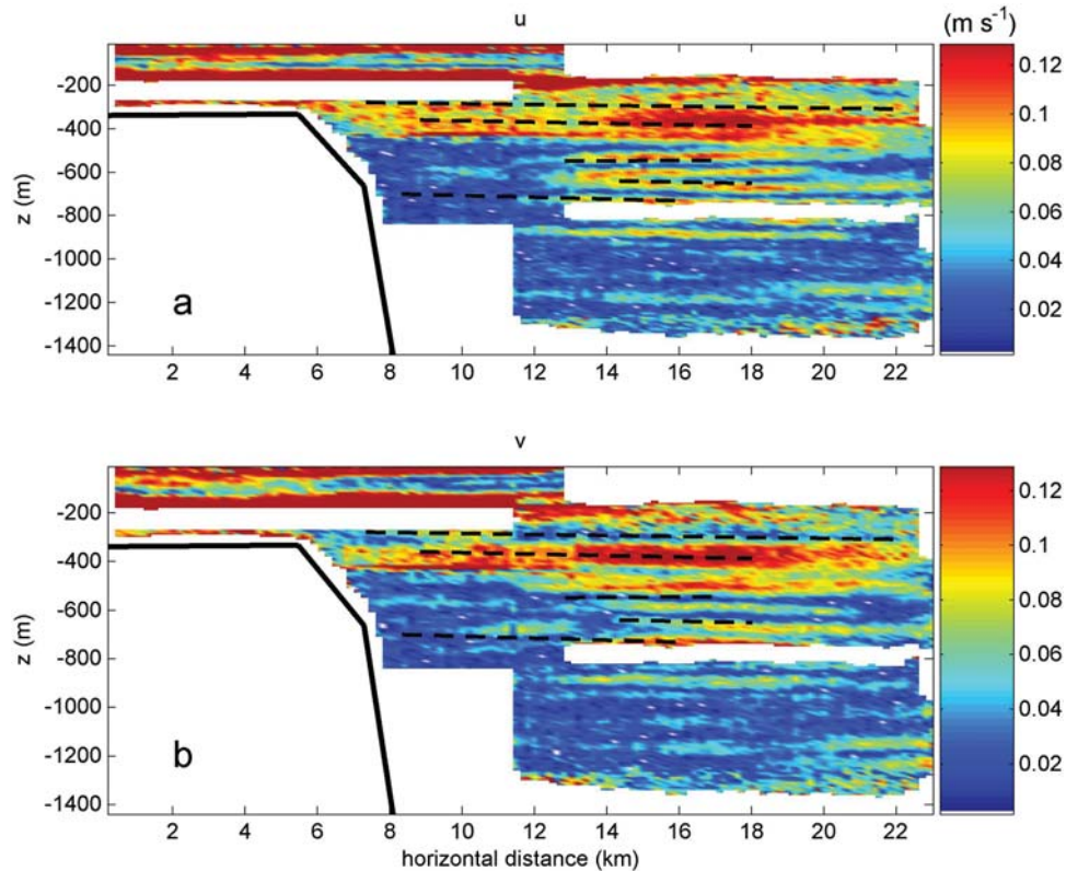
Figure 11. As Figure 9, but for diurnal motions. Note the difference color-scale compared to Figure 9.
