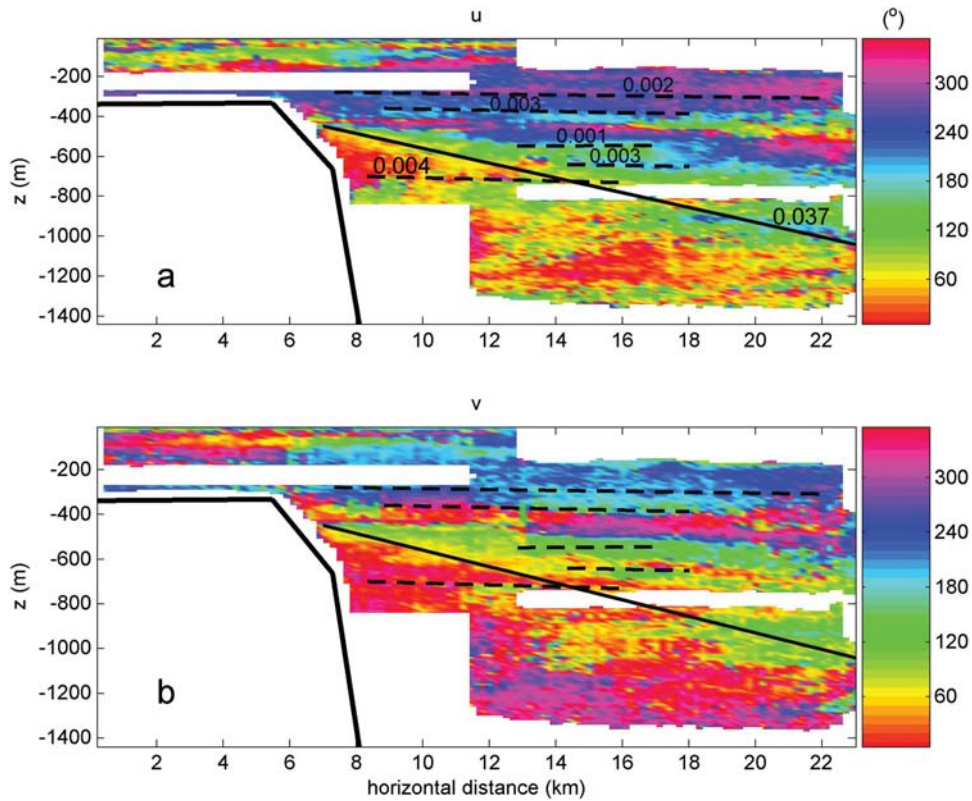
Figure 8. As Figure 5, but for GMS. Note that, as for BB, the theoretical solid and dashed curves (1), cf Table 1 and Figure 7b, are placed in rather arbitrary locations. They are valid for the entire domain and for Figures 8, 9, 10, 11 alike. The solid slope is for semidiurnal tidal motions in mean stratification or inertial motions in weak stratification (solid line, 0.037 (e.g., \sigma = M_2 , N = 45f and \sigma = 1.00f , N = 10f )). Sample dashed slopes may represent near-inertial or diurnal motions in moderately strong stratification or semidiurnal motions in extremely strong, N \approx 220f not observed, thin layer stratification (0.001 (e.g., \sigma = 1.00f , N = 60f ), 0.002 ( \sigma = 1.008f , N = 45f ), 0.003 ( \sigma = 1.01f , N = 30f and \sigma = 0.9999f , N = 34f ) and 0.004 ( \sigma = 1.00f , N = 30f and \sigma = 1.01f , N = 20f )).
