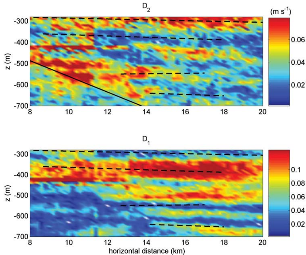
Figure 12. Zoom of Figure 9b (upper panel) and Figure 11b (lower panel): amplitudes of cross-slope motions above GMS for semidiurnal and diurnal/inertial frequencies, respectively. The straight solid (semidiurnal only) and dashed lines are identical in both panels and can be used for guidance to infer the alternating bands of enhanced/decreased amplitudes. Note the difference in color-scales.
