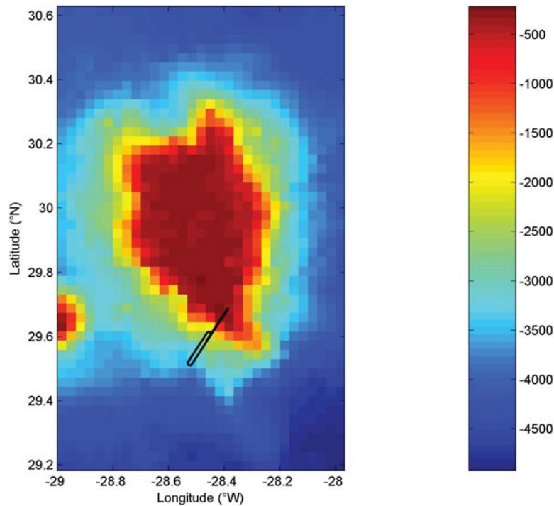
Figure 2. Great Meteor Seamount topography in the Canary Basin, with DTV-tracks consisting of a single shallow and a single deep portion. Colors indicate depth in m. Axes-direction as in Figure 1.
