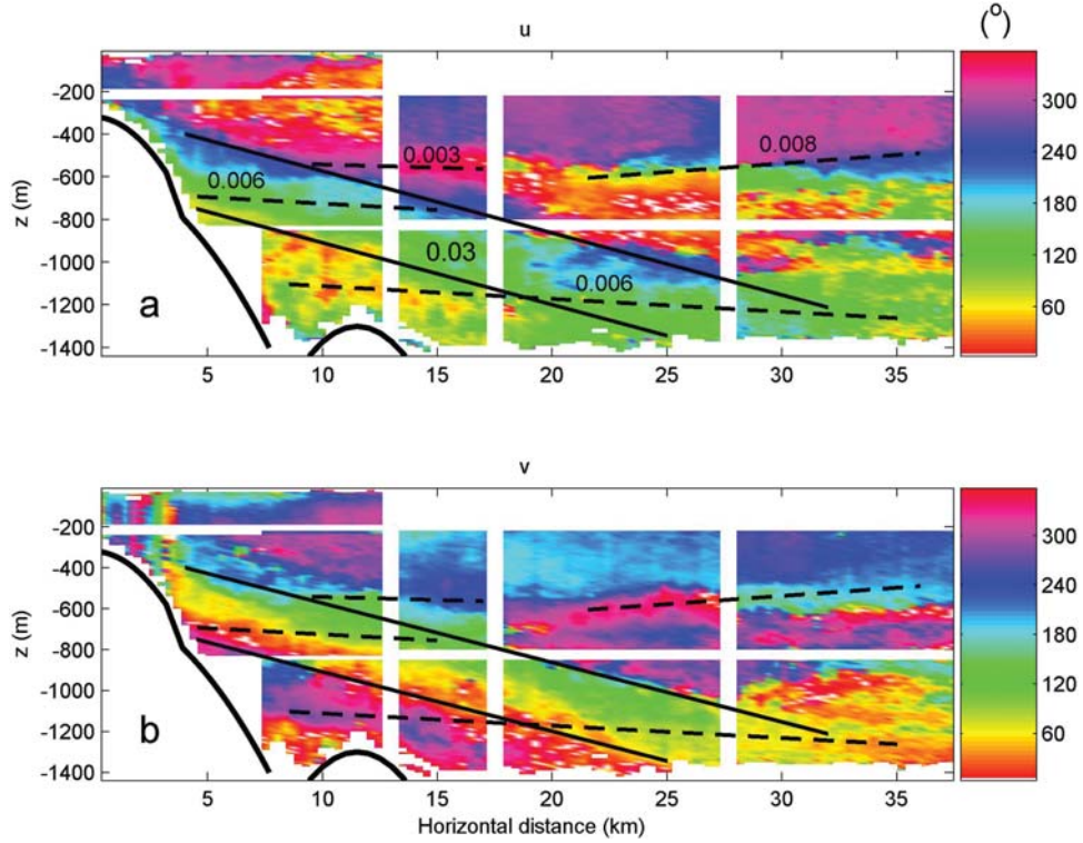
Figure 5. Semidiurnal tidal phase of (a) along-slope and (b) cross-slope component observed in BB.
