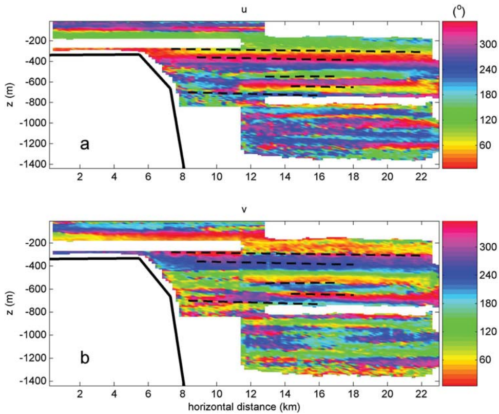
Figure 10. As Figure 8, but for diurnal motions.
