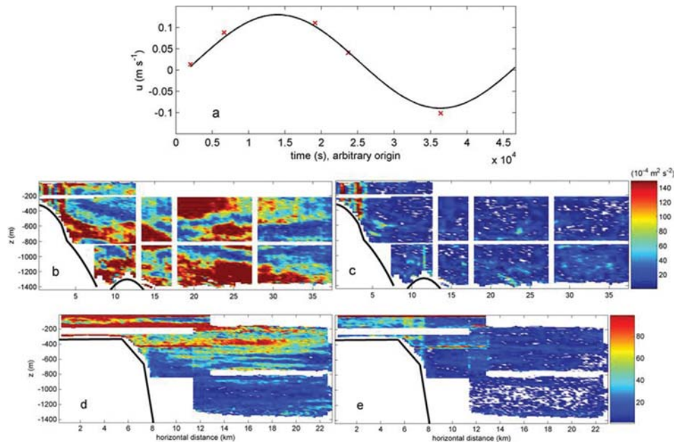
Figure 4. (a) Large-amplitude five-point data time series and its tidal harmonic fit, from BB. (b) Total variance of harmonic motions in cross-slope BB (colour scale as in (c)). (c) Rest-variance after subtraction of explained semidiurnal harmonic in cross-slope BB. (d) As (b), but for GMS (color scale as in (e)). (e) Rest-variance after subtraction of explained diurnal and semidiurnal harmonics in cross-slope GMS. Note the different colour-scale compared to BB.
