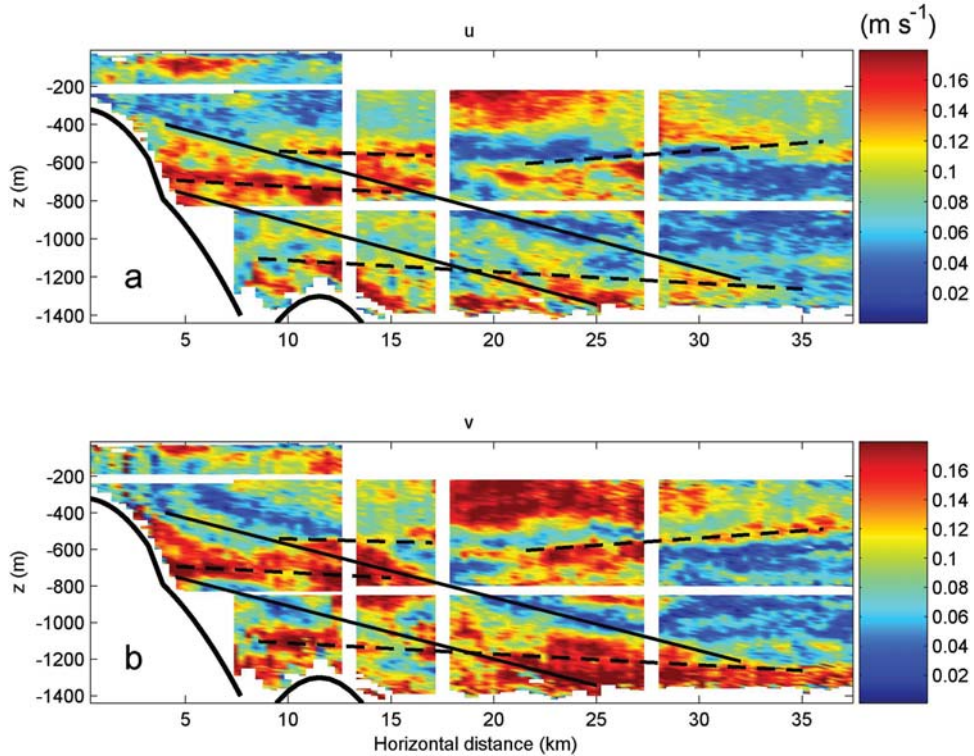
Figure 6. As Figure 5 but for the amplitude. The straight dashed and solid lines are identical to those in Figure 5.
