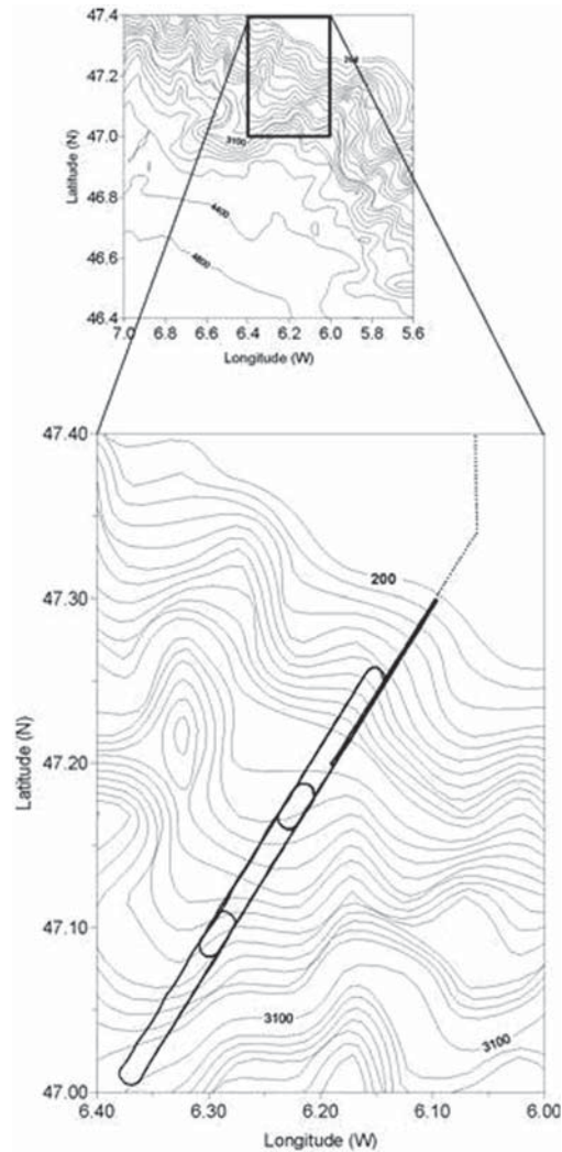
Figure 1. Part of the continental slope in the Bay of Biscay “BB” off Brittany (F), with the towed-ADCP “DTV” tracks superposed in the detail. Depth in m. The wide tracks are “deep,” when DTV is at 800 m, the narrow track “shallow,” when the DTV is at 200 m. Along-slope x-axis is positive to the North-west, y-axis is positive off-slope.
