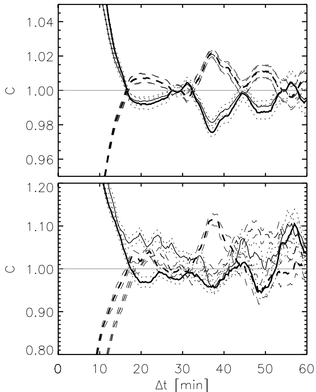
Fig. 1. Persistence of granules and intergranular lanes, measured as spatial correspondence C between various G brightness classes as function of elapsed time \Delta t . The value C = 1 implies absence of spatial alignment, C > 1 preferential co-location, C < 1 spatial avoidance. The upper panel is for granules and lanes, the lower panel for the extreme subclasses made up by bright granules and dark lanes (see text). Thick solid curves: spatial correspondence between pixels belonging to granules and pixels that belong to granules \Delta t later (upper panel), and similarly for bright granules (lower panel). Thin solid curves: similarly between lanes and subsequent lanes (upper panel) and between dark lanes and subsequent dark lanes (lower panel). Thick dashed curves: similarly between lanes and granules (upper panel) or dark lanes and bright granules (lower panel), with the lanes observed before the granules. Thin dashed curves: similarly but with the granules observed before the lanes. One-sigma error estimates are added to each curve (dotted or dashed)
