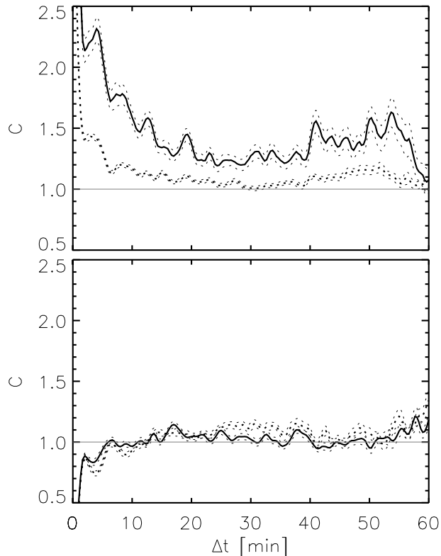
Fig. 2. Ca II K brightness persistence, measured as spatial correspondence C between two K brightness classes as function of elapsed time \Delta t . The upper panel shows the persistence of bright K pixels (solid curve) and of dark K pixels (dashed curve). The lower panel measures the time-delay correspondence between bright K pixels and dark K pixels, with the solid curve for sampling bright after dark and the dashed curve for sampling dark after bright
